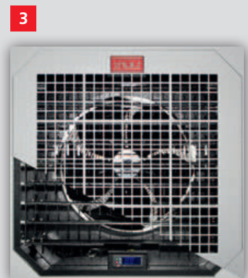
AirBooster Pro with adjustable air transfer grille and variable speed EC fan
