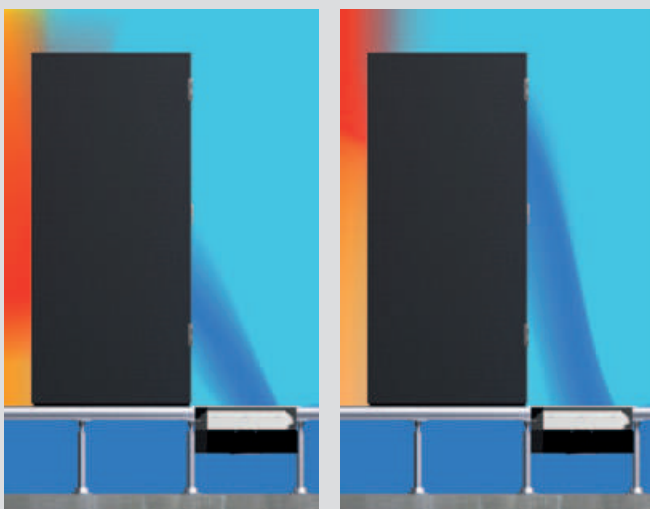
Manually adjustable air transfer grilles allow air flow to be directed to the most heat-stressed areas, depending on server rack equipment
